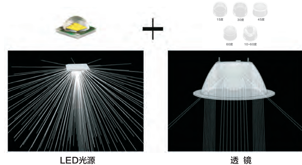
Focus Reflection光学控光原理
